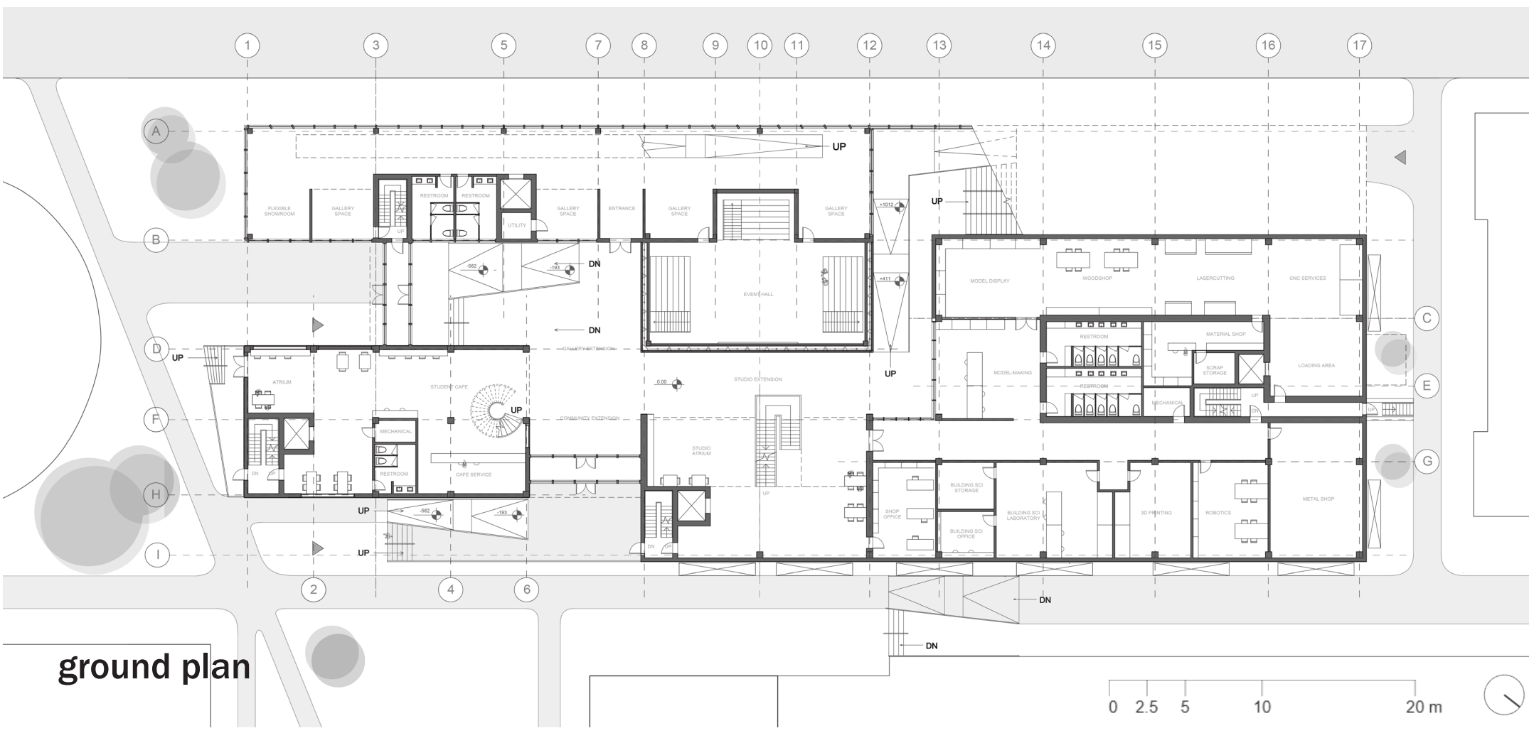
context plan
